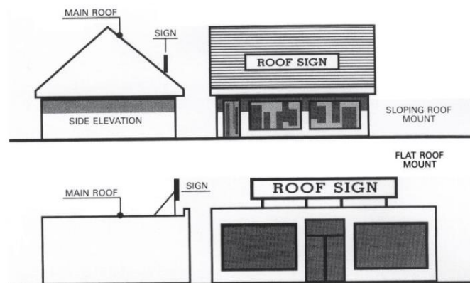
Figure 30.07-18: Roof Sign
