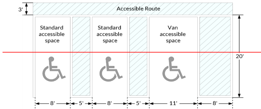
Figure 30.04-4: Accessible Space and Access Design
